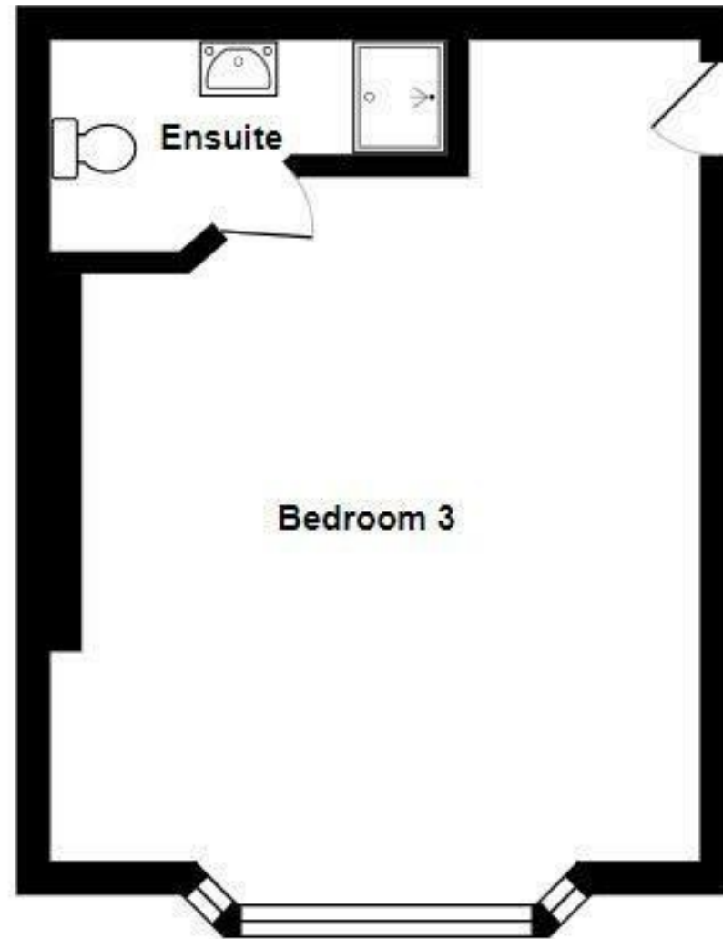
Ground Floor - Bedroom 3
